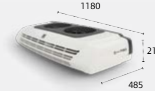
C-450/C-550/C-650/C-750 CONDENSER
