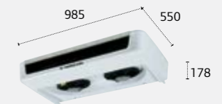
ES300 ULTRA SLIM EVAPORATOR
